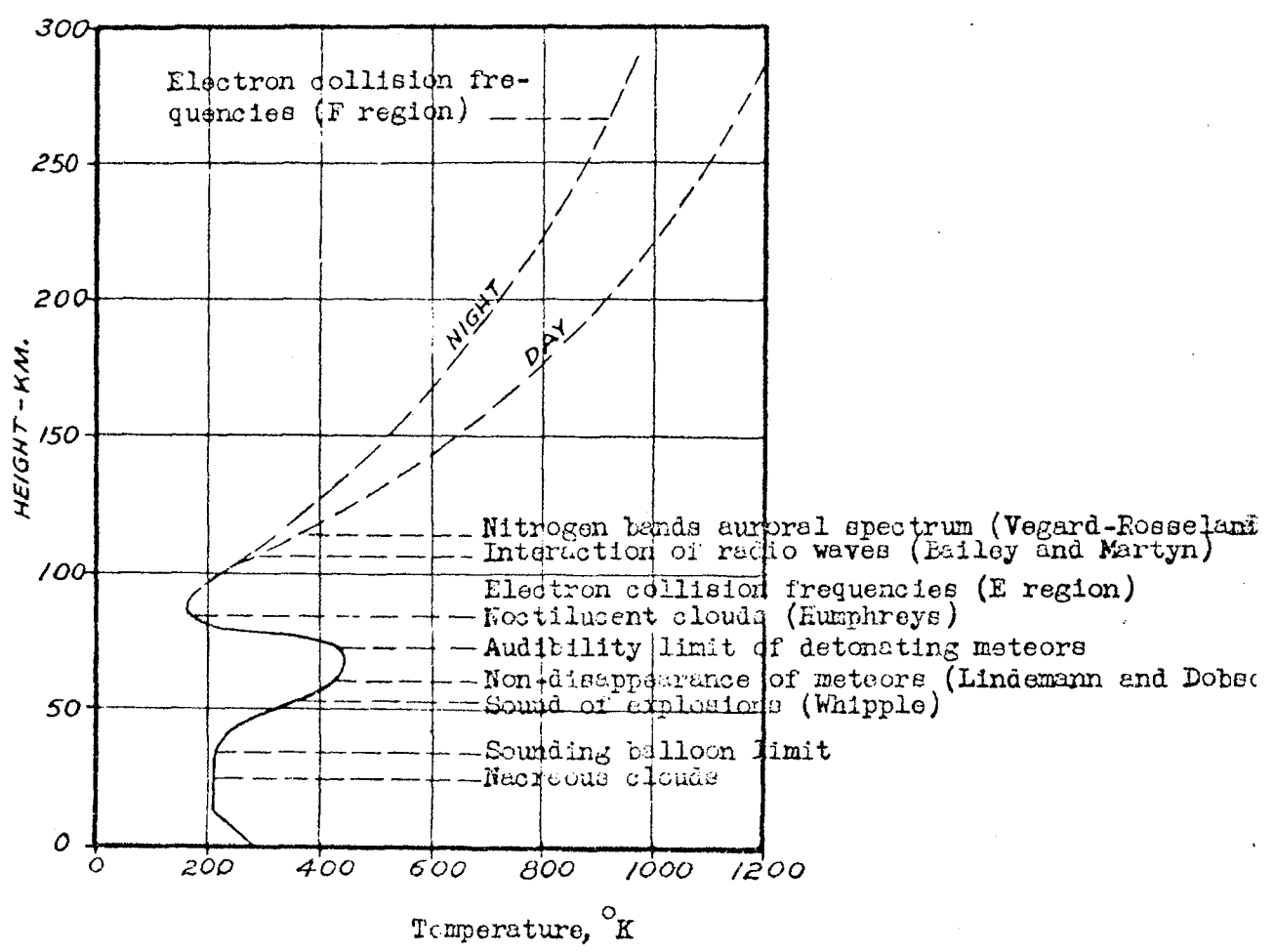
Fig. 1 Temperature Distribution in the Upper Atmosphere According to Martyn and Pulley (Ref. 7).
