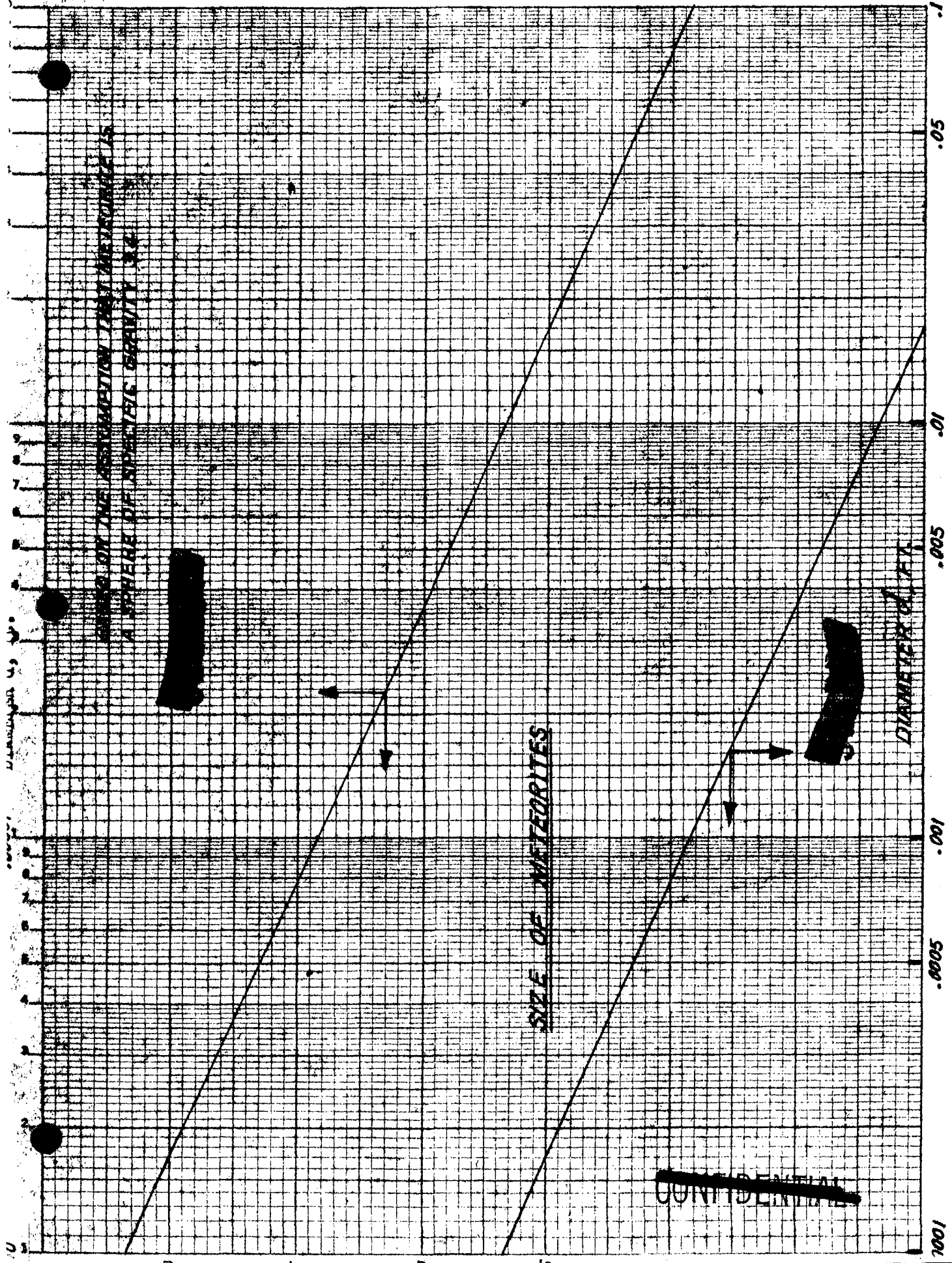
FIG. 1 SIZE OF METEORITE CORRESPONDING TO METEOR MAGNITUDE. SEE TABLE 2.
