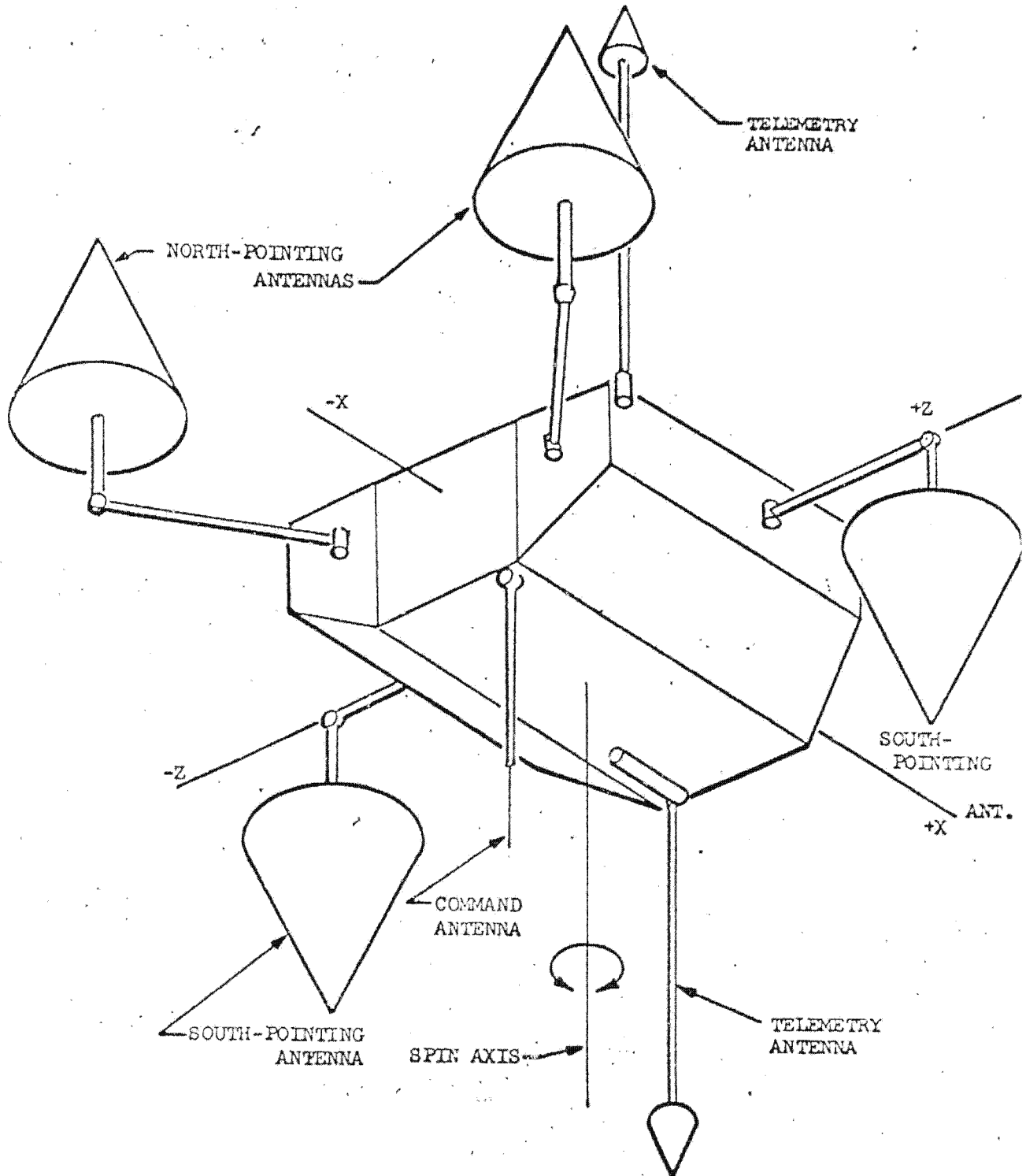
Figure 2-1 Antenna Subsystem
