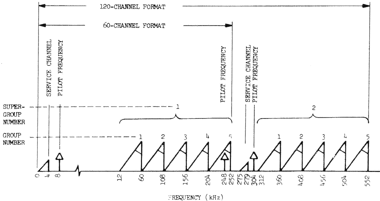
Figure 1-9 120-Channel FDM Format in the 700- to 1000-MHz Band
