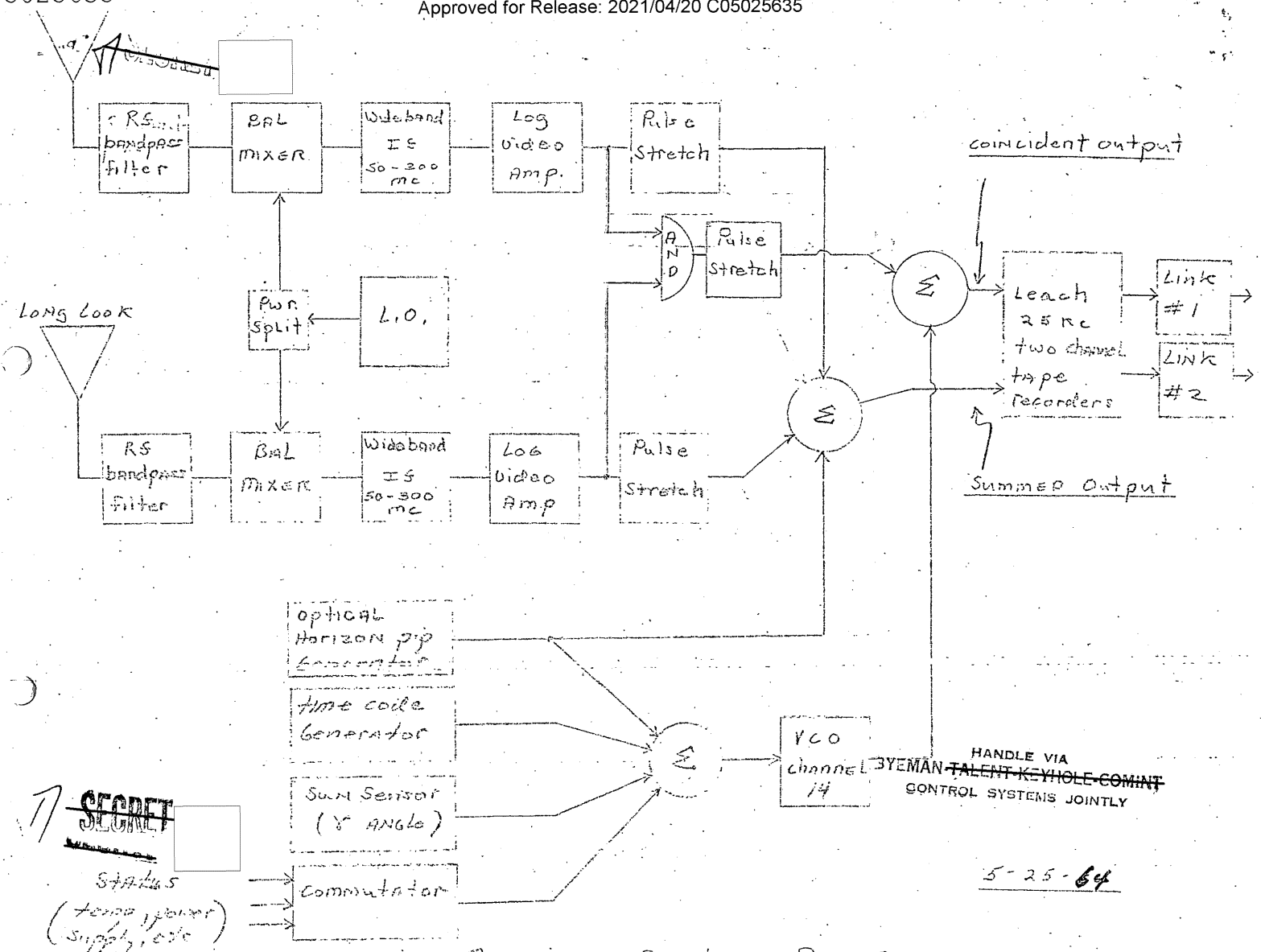
FANION Receiver System Diagram
