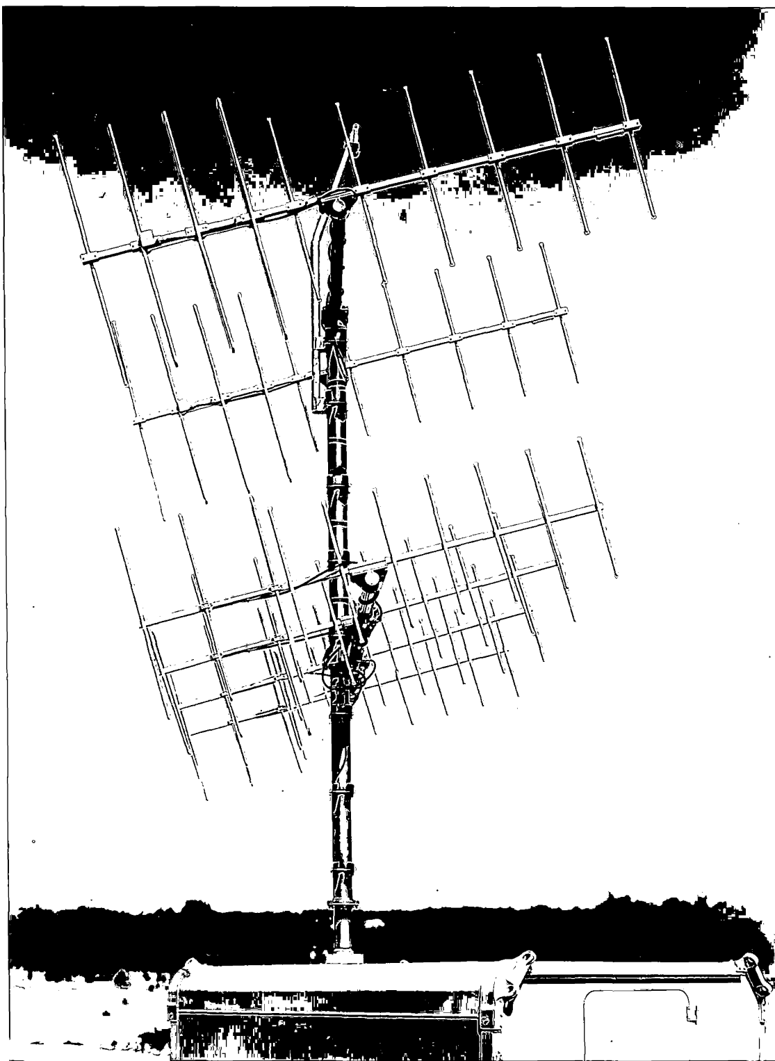
Fig. 1 Antenna Mast.
