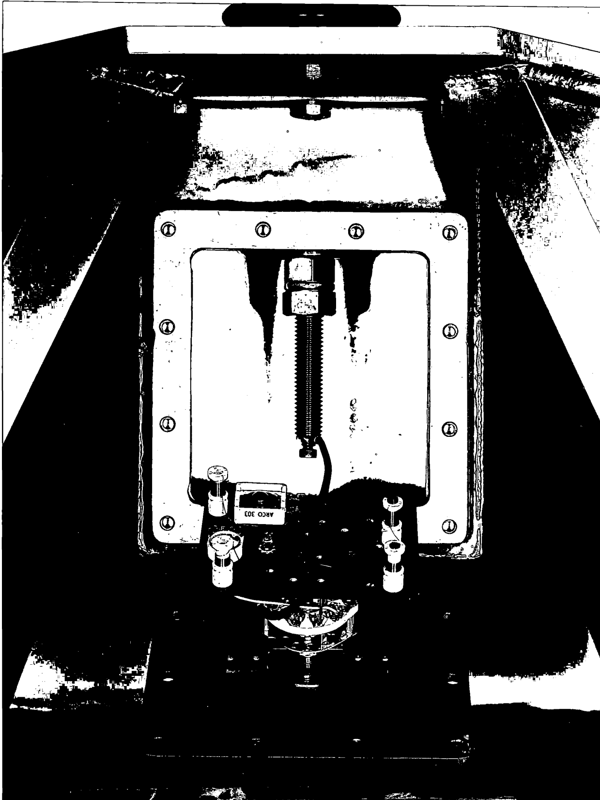
Fig. 10 Whip Antenna Transformers
