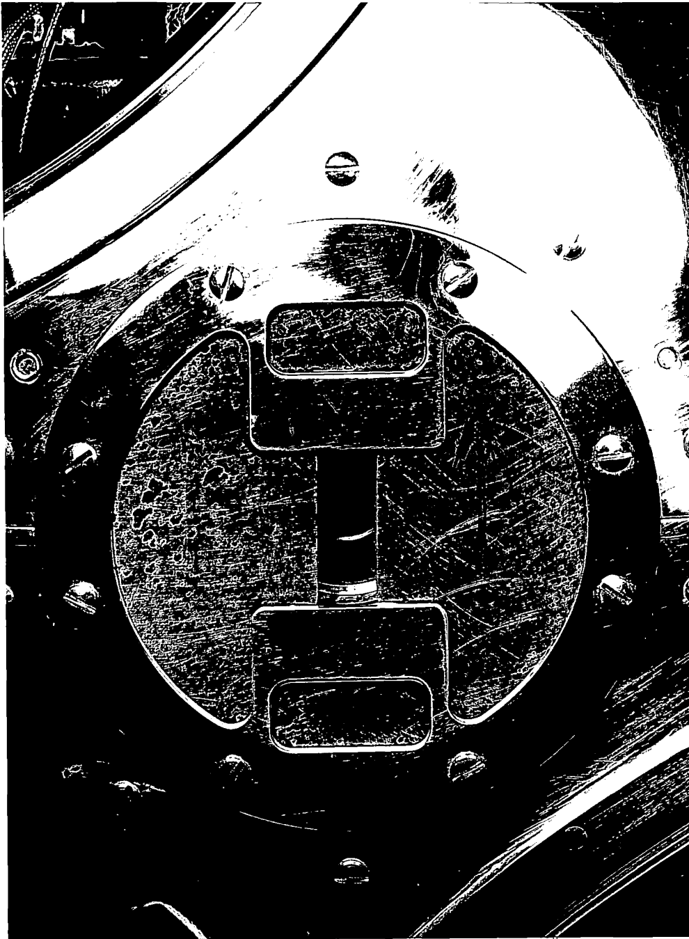
Solar Radiation II, Flight Unit #1 showing magnet and X-Ray sensor with SR I type magnet cover plate before aluminum paint was applied and sensor changed 28 October 1960
