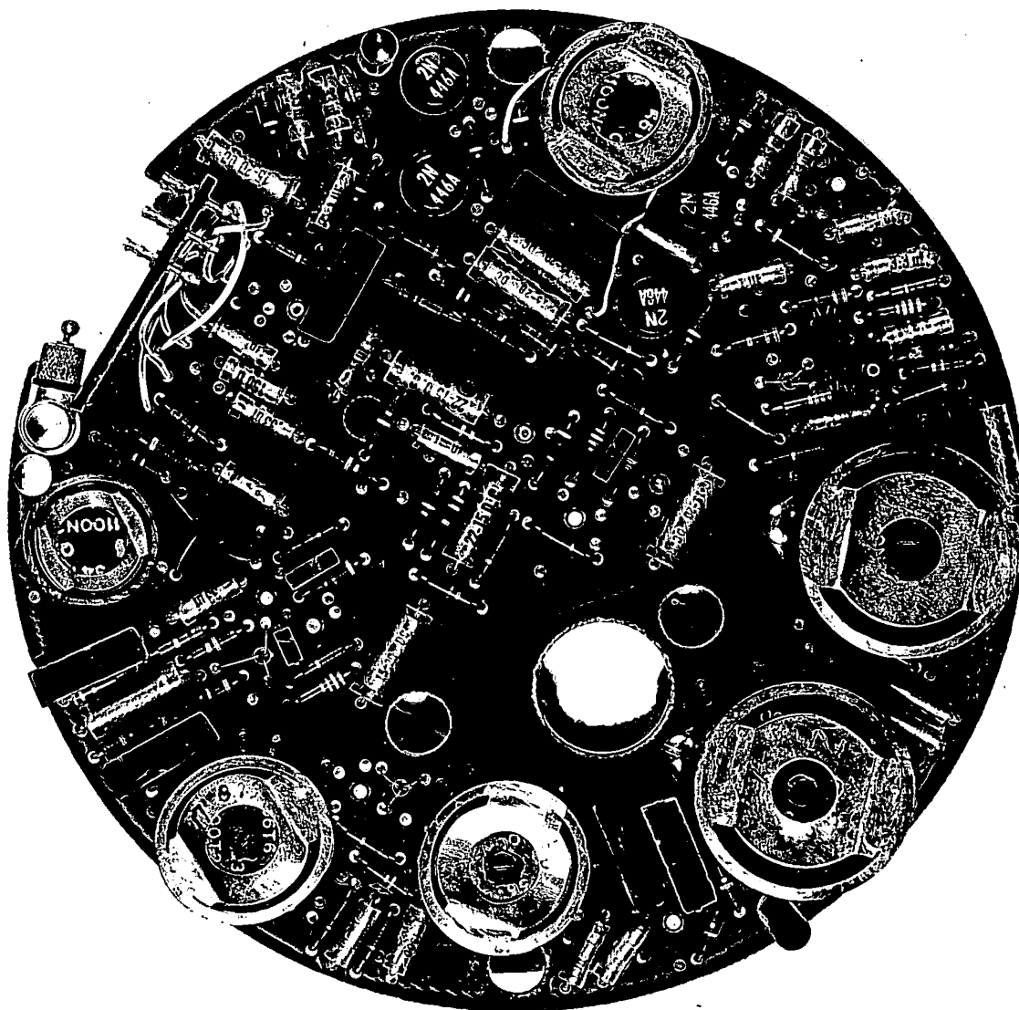
VLF Receiver Signal Card Top View
