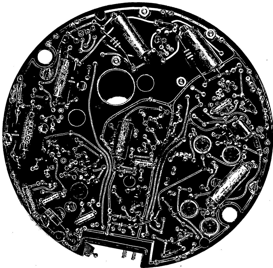
VLF Receiver Signal Card Bottom View
