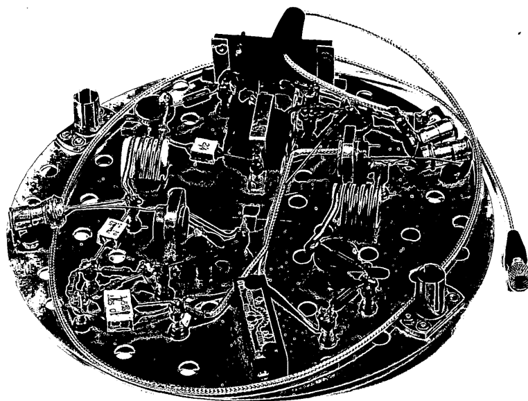
108 mc 30 mw DuKane Transmitter
