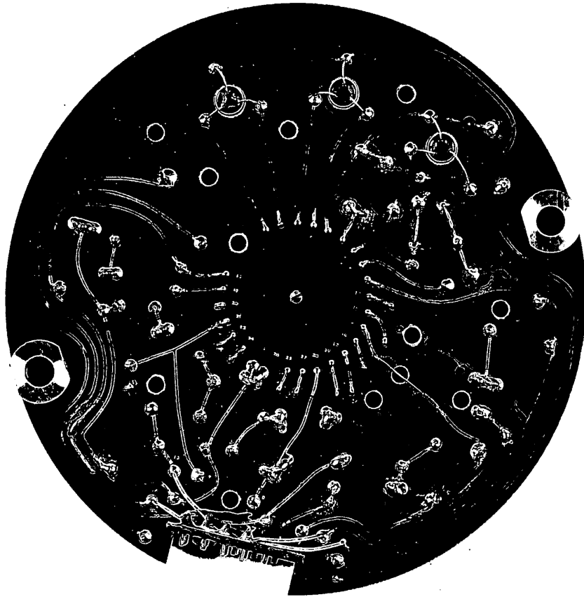
Power Supply for Lyman-Alpha-XRay and Aspect Amplifiers (Card L)
