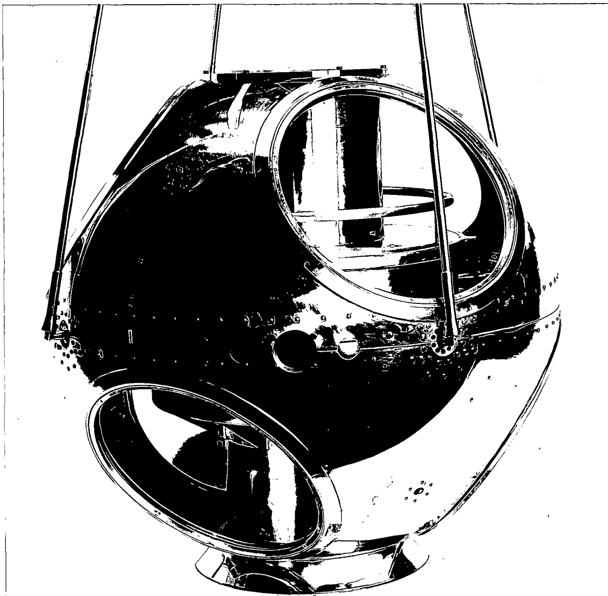
Prototype Structure Solar Radiation Satellite (Side view showing Lyman-Alpha & Aspect Sensor Mount) 23 February 1960
