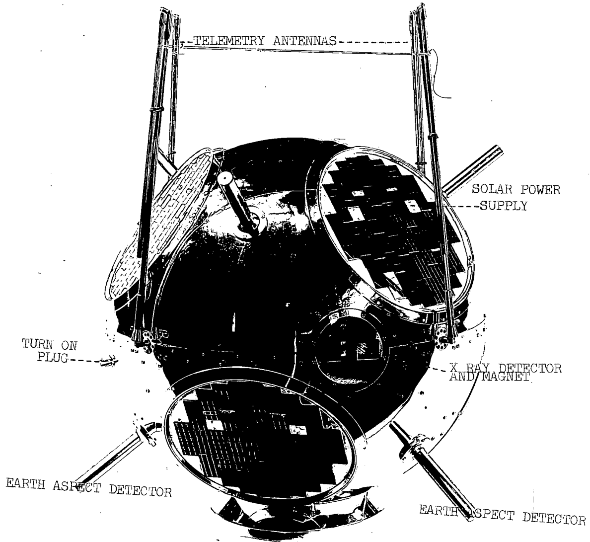
SOLAR RADIATION III SATELLITE x(xixfxixix AS CONTAINED IN NOSE FARING
