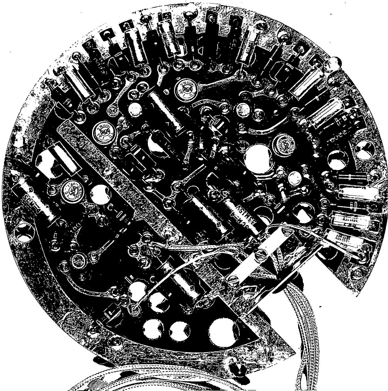
Data Link Amplifier Solar Radiation III May 1961
