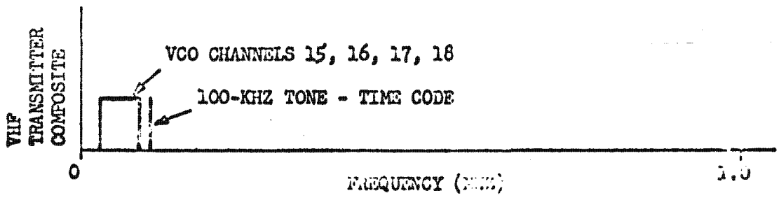
DIAGRAM 4. Frequency Modulation
