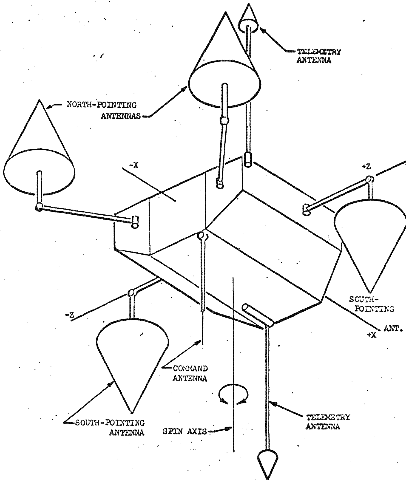
Figure 2-1 Antenna Subsystem
