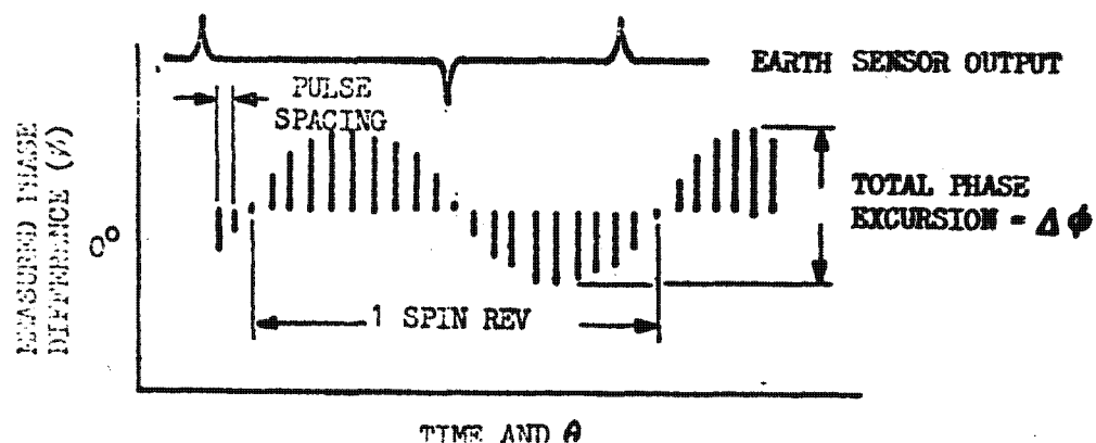
DIAGRAM 2. Phase Measurement Geometry
