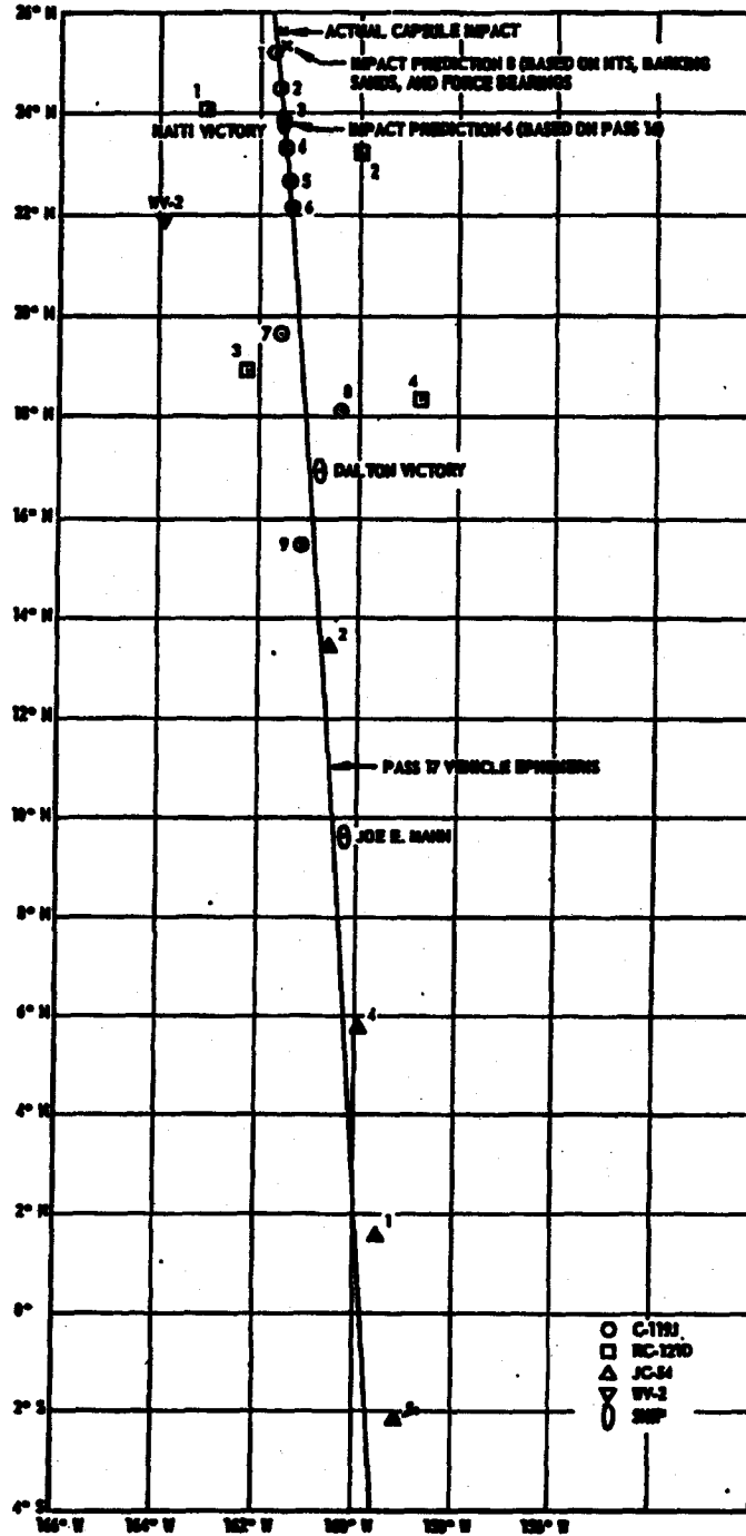
Figure 5 Recovery Force Deployment of ETPD
