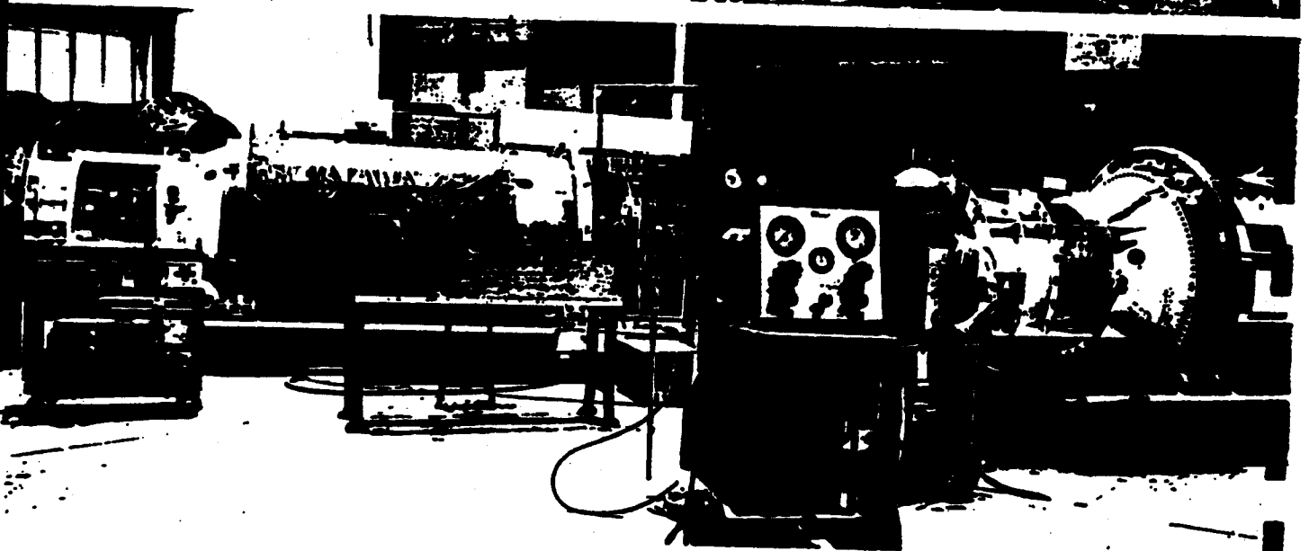
Figure 3. Change-over from AGENA "A" to AGENA "B" in the missile assembly building at Vandenberg Air Force Base. The AGENA "A" on the right, is DISCOVERER XV which was launched on 13 September. One more AGENA "A" remains to be flown. On the left is the AGENA "B" vehicle scheduled for launch in October as DISCOVERER XVI.
