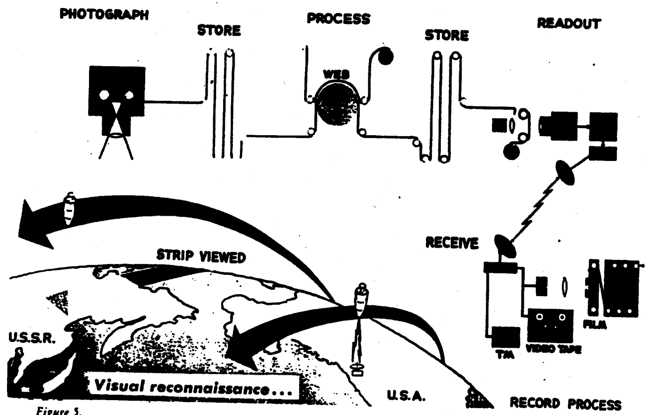
Figure 5. The initial visual reconnaissance program will use conventional photo techniques with automatic film processing and TV-type electronic image readout to ground stations thru a data link. Ground electronics will reconvert the signal into photo image form, with a capability of resolving objects 20 feet in length.
