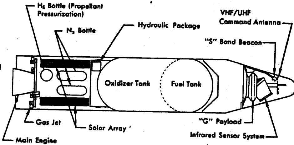
MIDAS, Configuration II, AGENA "B" Satellite
