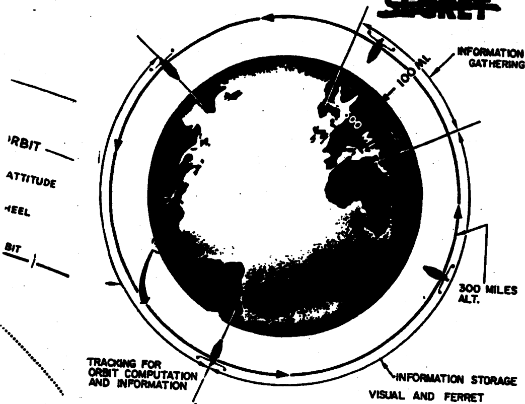
Figure 3. Schematic of SAMOS system in operational orbit. When the satellite is over the area of interest the sensing equipment is turned on (Information gathering). When it leaves the area of interest the sensing equipment is turned off and the sensing data is processed (Information storage). When the vehicle comes within range of a ground receiving station, the data will be read-out upon command for processing and transmitted to using agencies. This process is continuously repeated during the useful lifetime of the vehicle.
