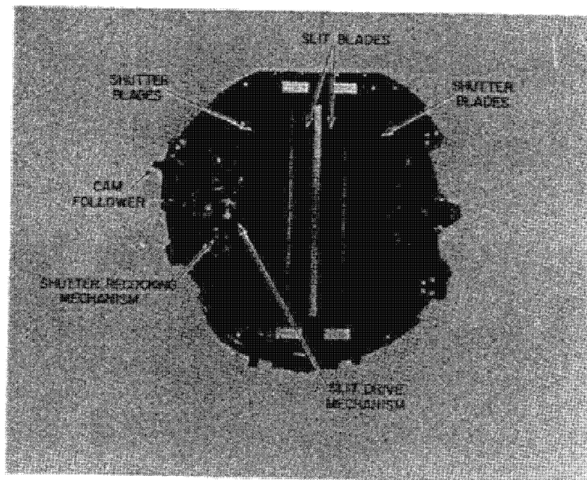
Slit and Shutter Assembly
