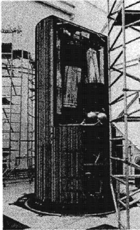
Midsection Assembly Installed on Shaker Cluster
