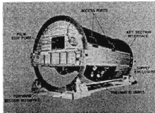
Mid-Section of the Hexagon Camera System
