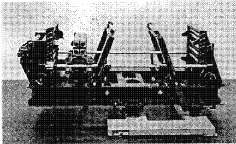
Looper Assembly (SV-1 through SV-16 Configuration)
