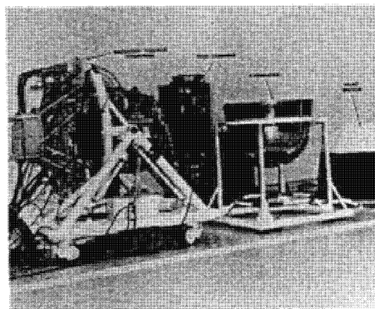
Test Set-up for Take-Up Assembly
