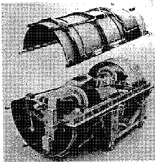
Thermal Model
