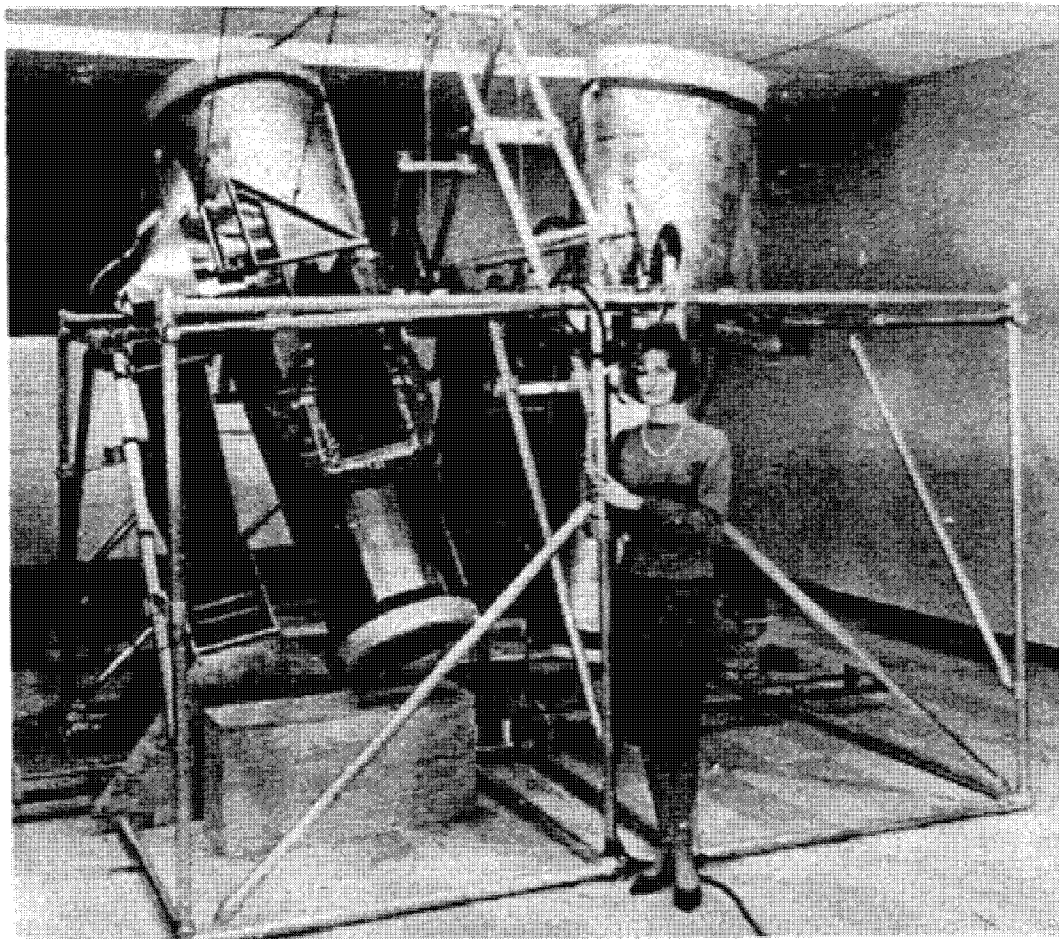
Full scale mockup of Perkin-Elmer's Phase I design. Due to its configuration and operation, it was nicknamed the "cocktail shaker." It contained a film transport system consisting of rollers and air bars, and transferred film from a supply spool to a take-up spool.
