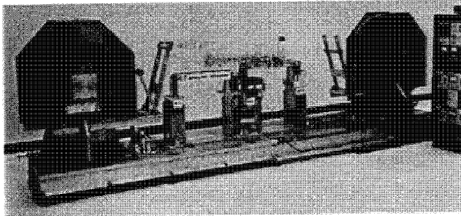
Forward Articulator Test Bed
