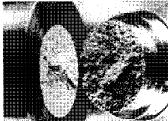
End View of Beryllium Shaft Fracture (10X)
