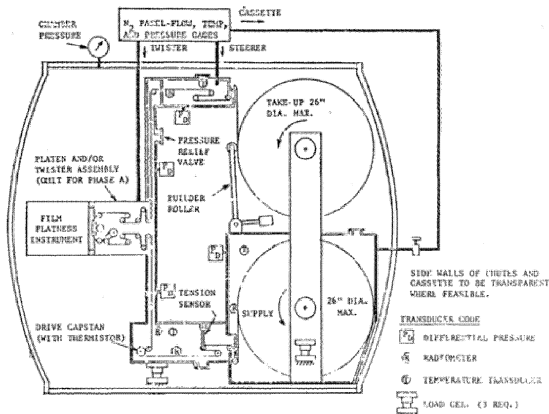
Abbreviated Film Path Schematic
