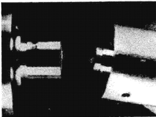
Side View of Beryllium Shaft Fracture (3.5X)
