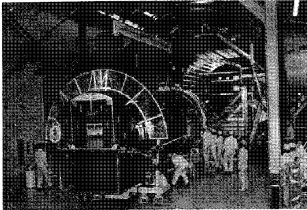
Engineering Model Installation into Chamber A
