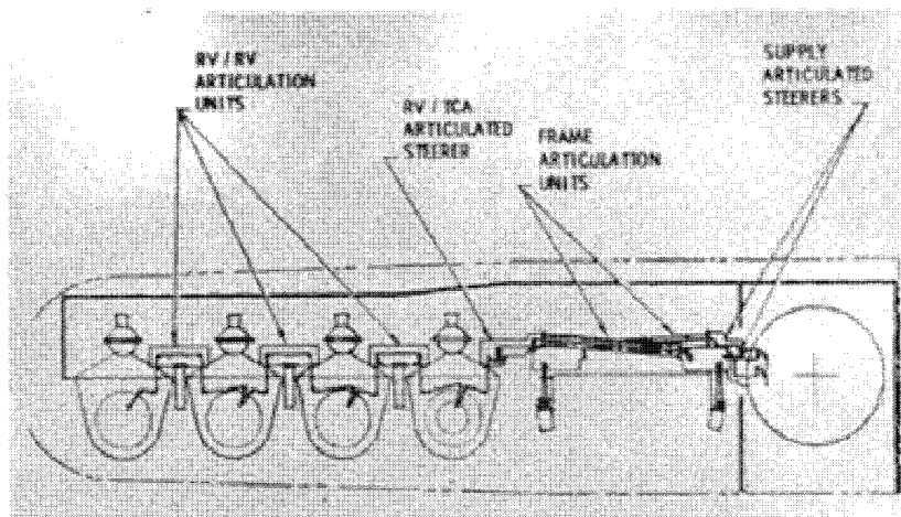
Articulation Units in Sensor Subsystem
