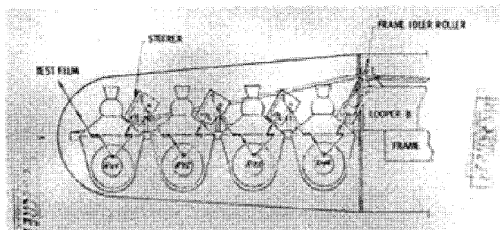
Early Conceptual Drawing of 4-RV Arrangement in Forward Section
