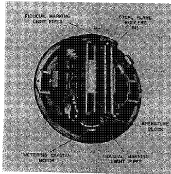
Front View of Platen Assembly
