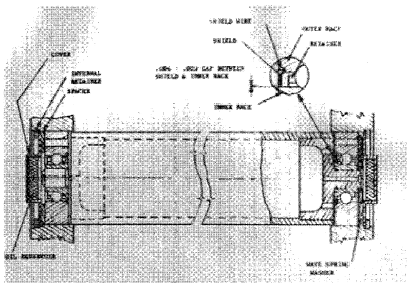
"Standard" Film Roller Design
