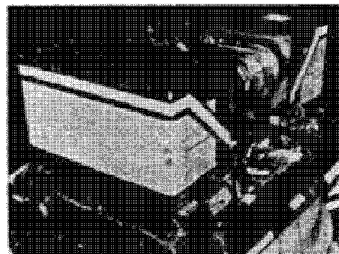
Passive Articulator Qualification Vibration Test
