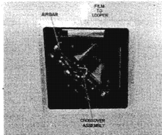
Flight Model, Crossover Assembly
