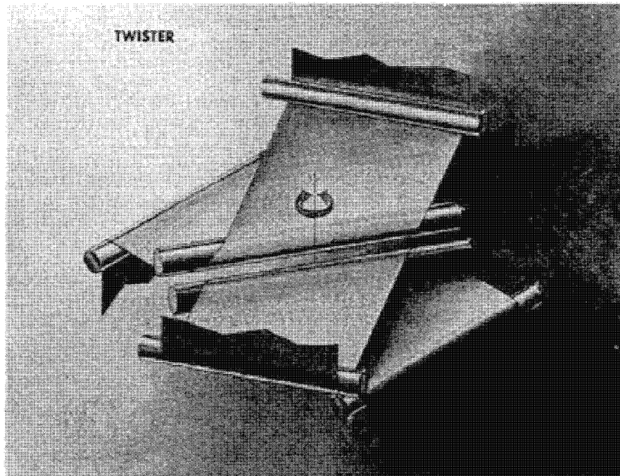
The Air Bar Twister Device
