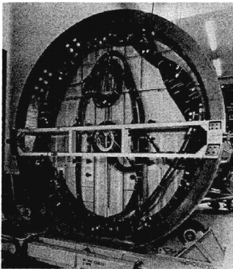
Cabling Arrangement at Aft End of Midsection
