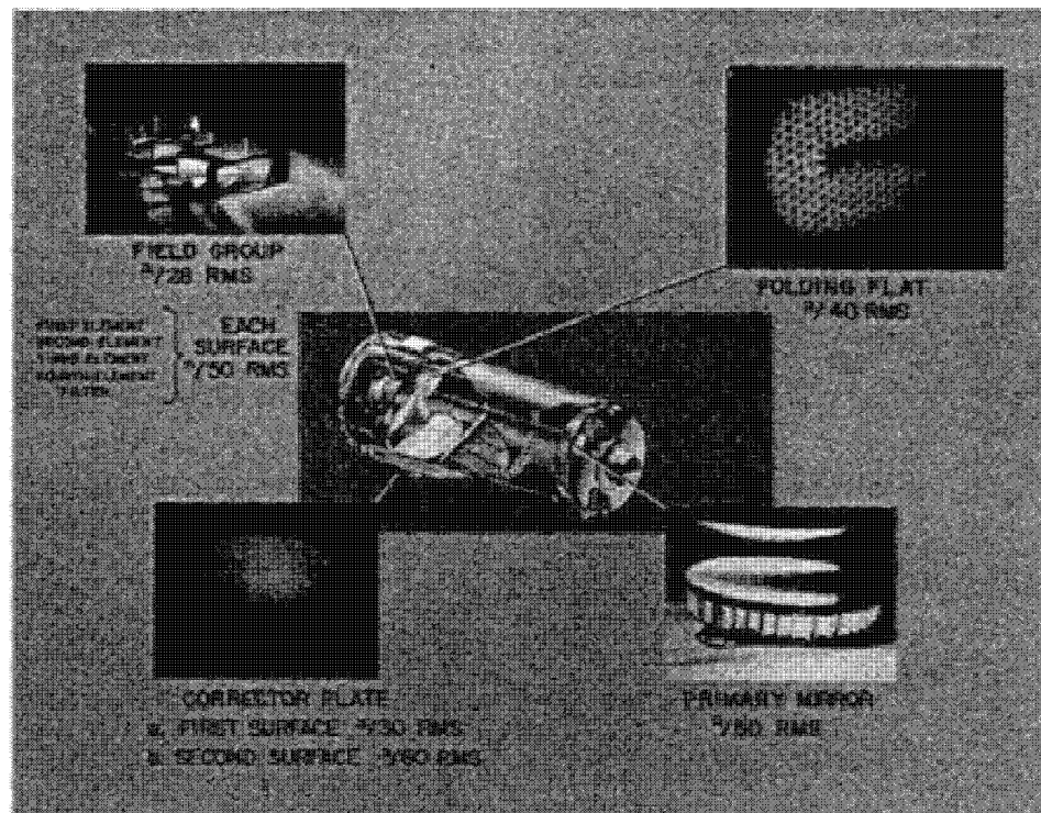
Hexagon Optical System Components
