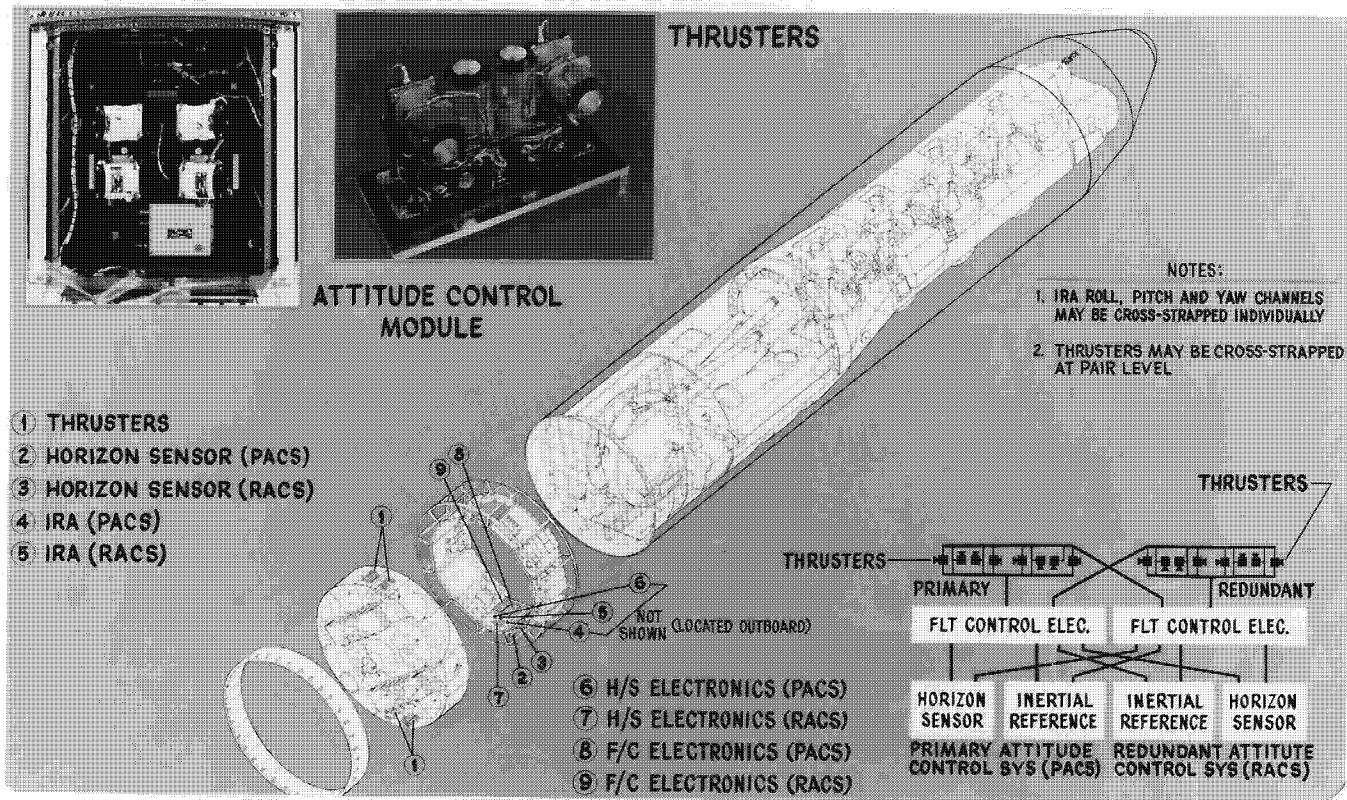
Fig. 1-7 — Attitude control
