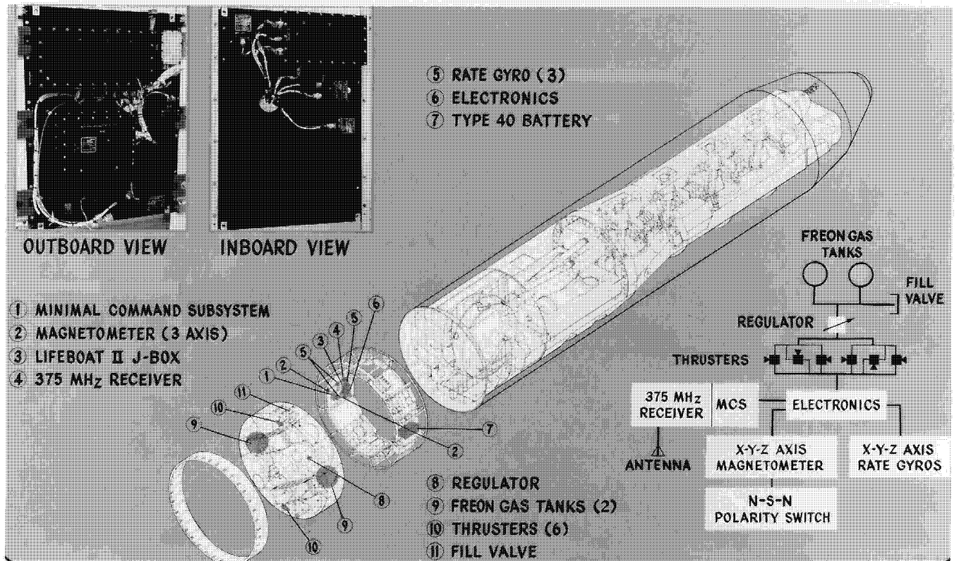
Fig. 1-12 — Lifeboat II
