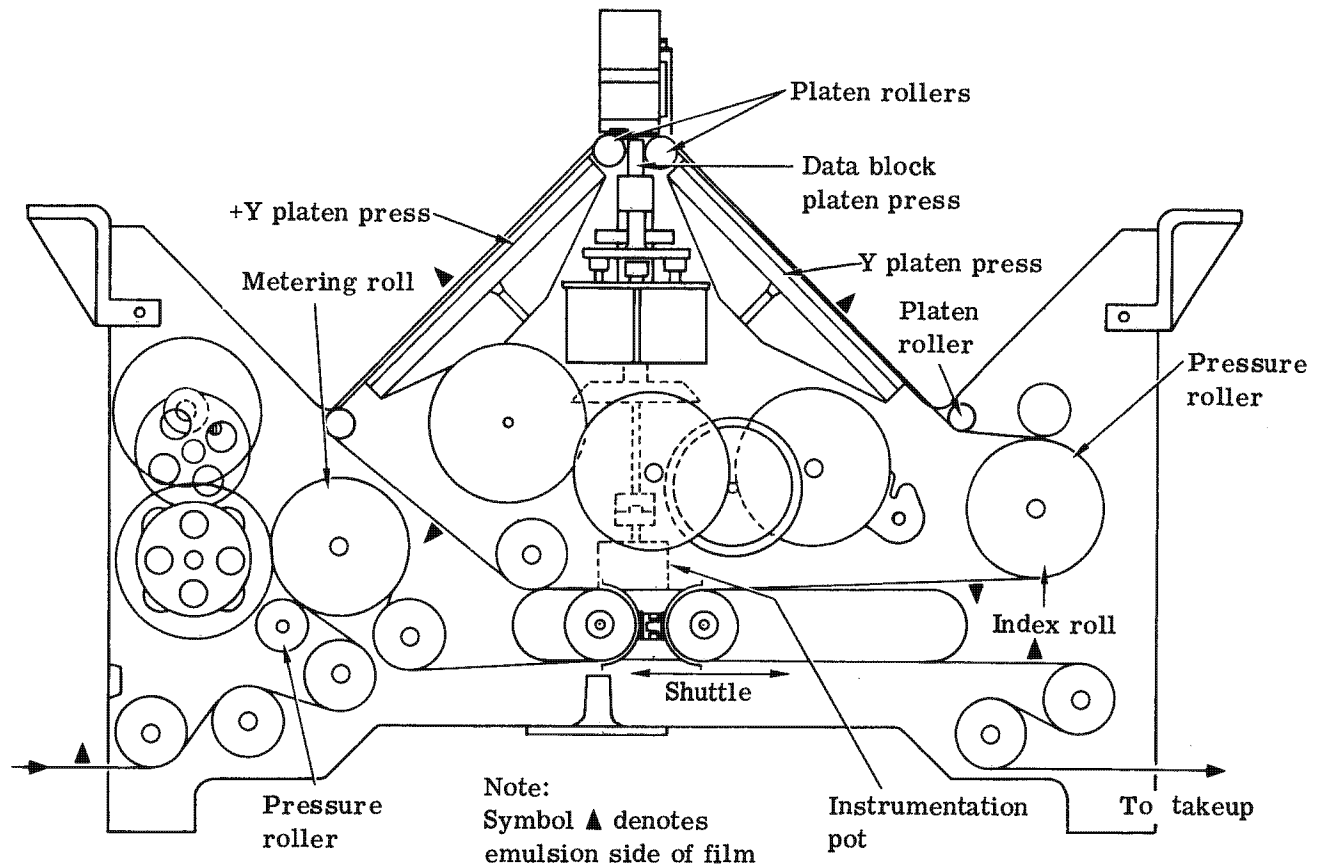
Fig. 2-18 — Stellar transport film flow
