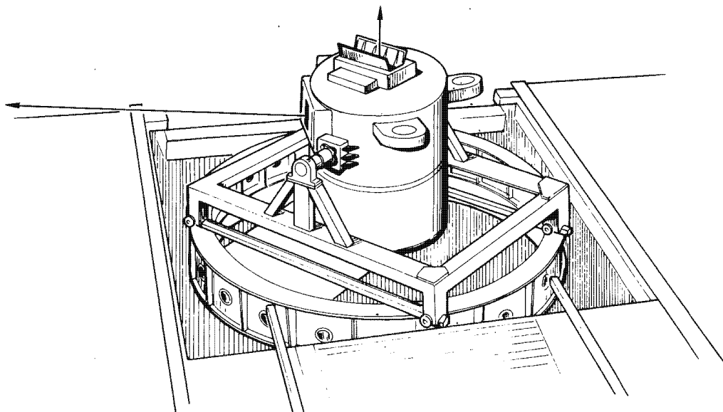
Fig. 2-24 — Cloudcroft calibration enclosure
