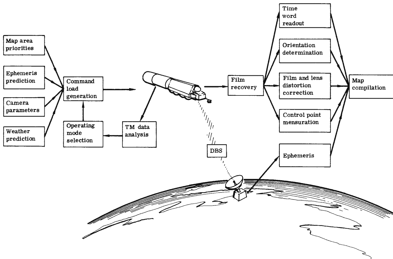
Fig. 3-7 — Mapping Camera operational data flow
