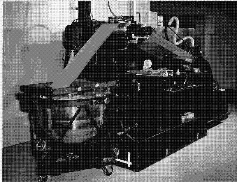
Fig. 4-3 — SRV interfaced with presplice complex
