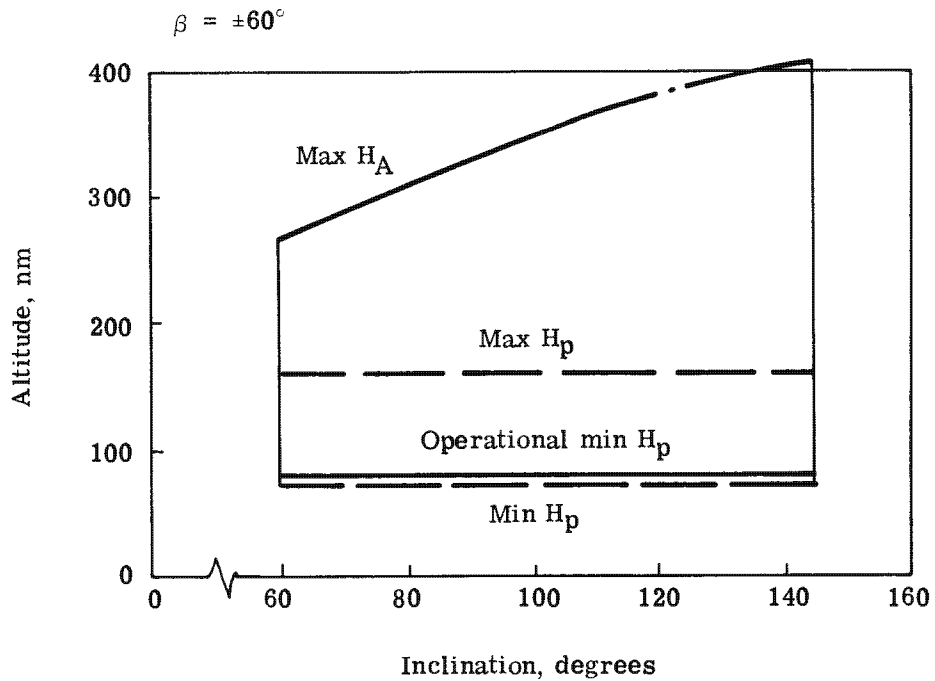
Fig. 1-18 — Mission flight envelope
