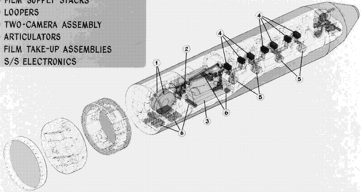
Fig. 1-13 — Search/surveillance cameras
