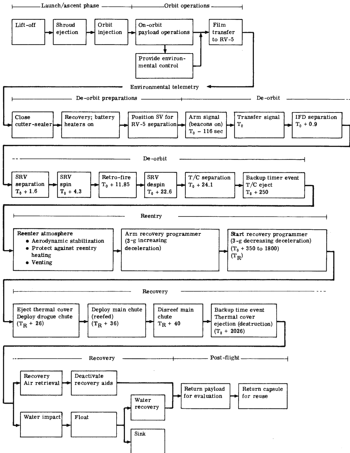
Fig. 1-21 — Mission flow
