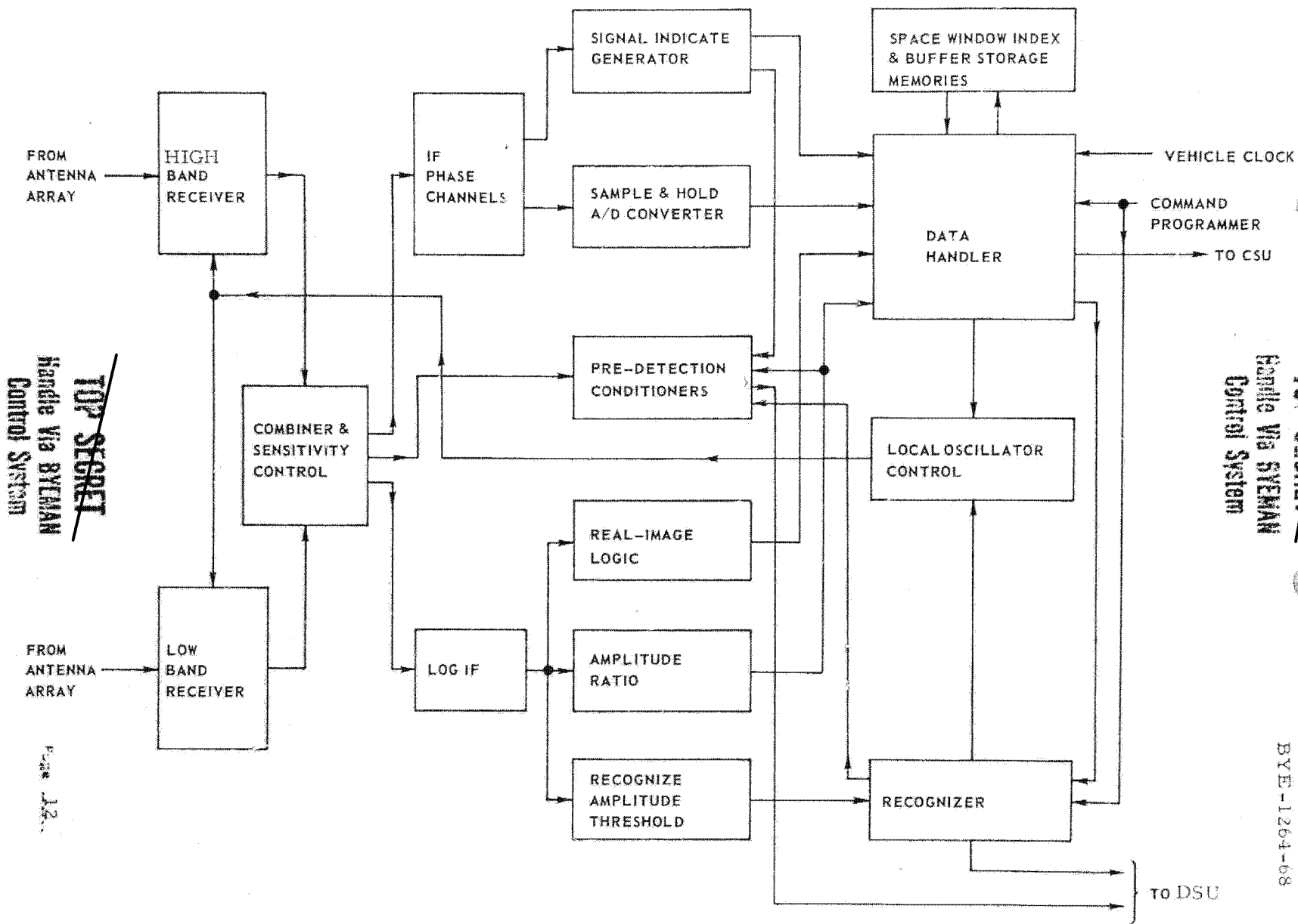
DIAGRAM 2 BLOCK DIAGRAM OF REAPER PAYLOAD
