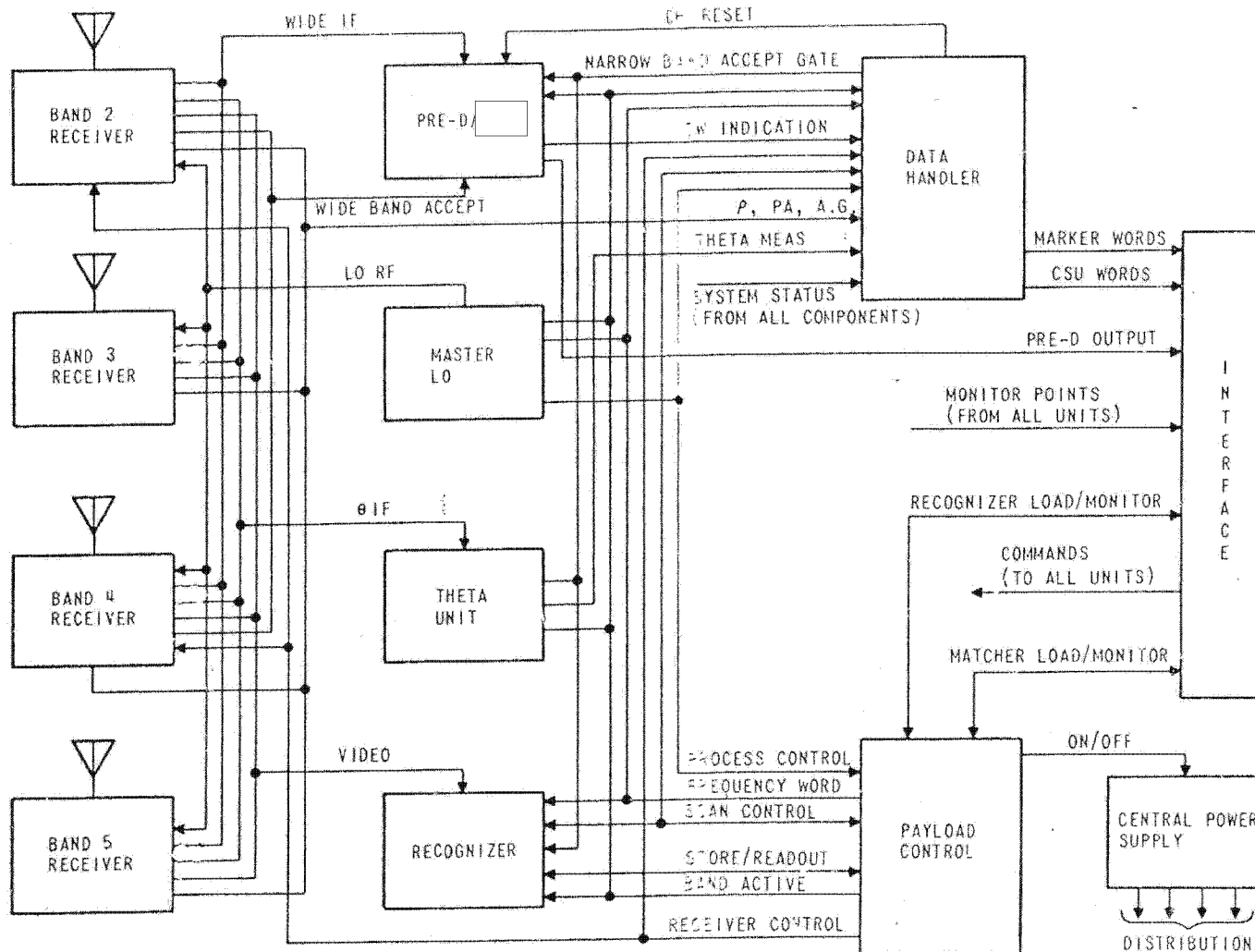
DIAGRAM 1. BLOCK DIAGRAM OF THRESHER PAYLOAD
