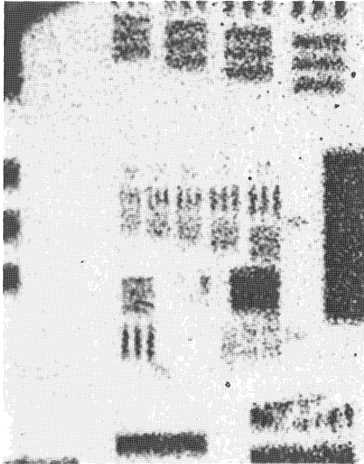
USAF 1951 TARGET
