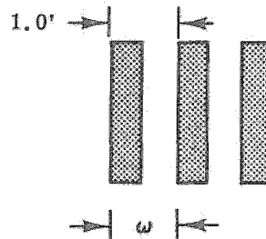
TRIBAR TEST TARGET ELEMENT ON THE GROUND
