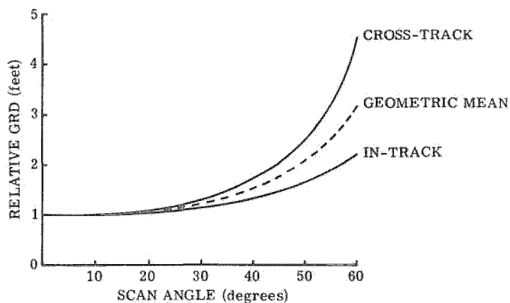
RELATIVE GROUND RESOLVED DISTANCE VERSUS SCAN ANGLE OF A HORIZONTAL OBJECT (90.8 NM)
