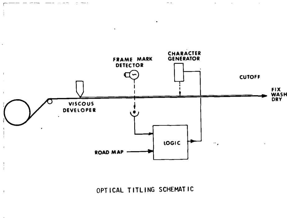
FIGURE 27 - Optical Titling Schematic
