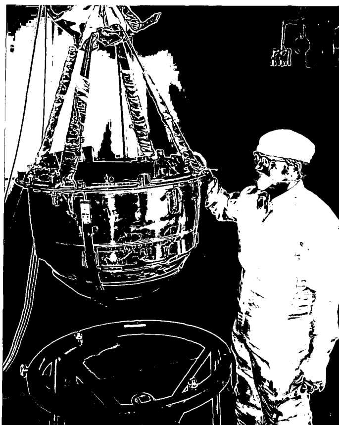
FIGURE 21 - Gambit SRV
