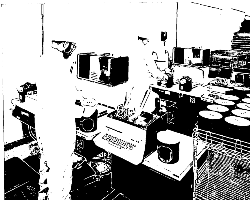
FIGURE 41 - Labeling Station
