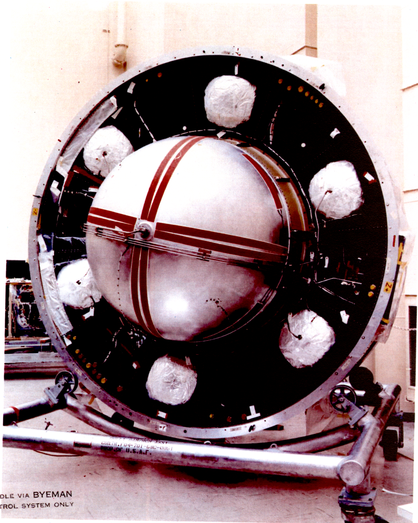
FIRST FLIGHT ORBIT ADJUST MODULE/REACTION CONTROL MODULE (LOOKING AFT)
