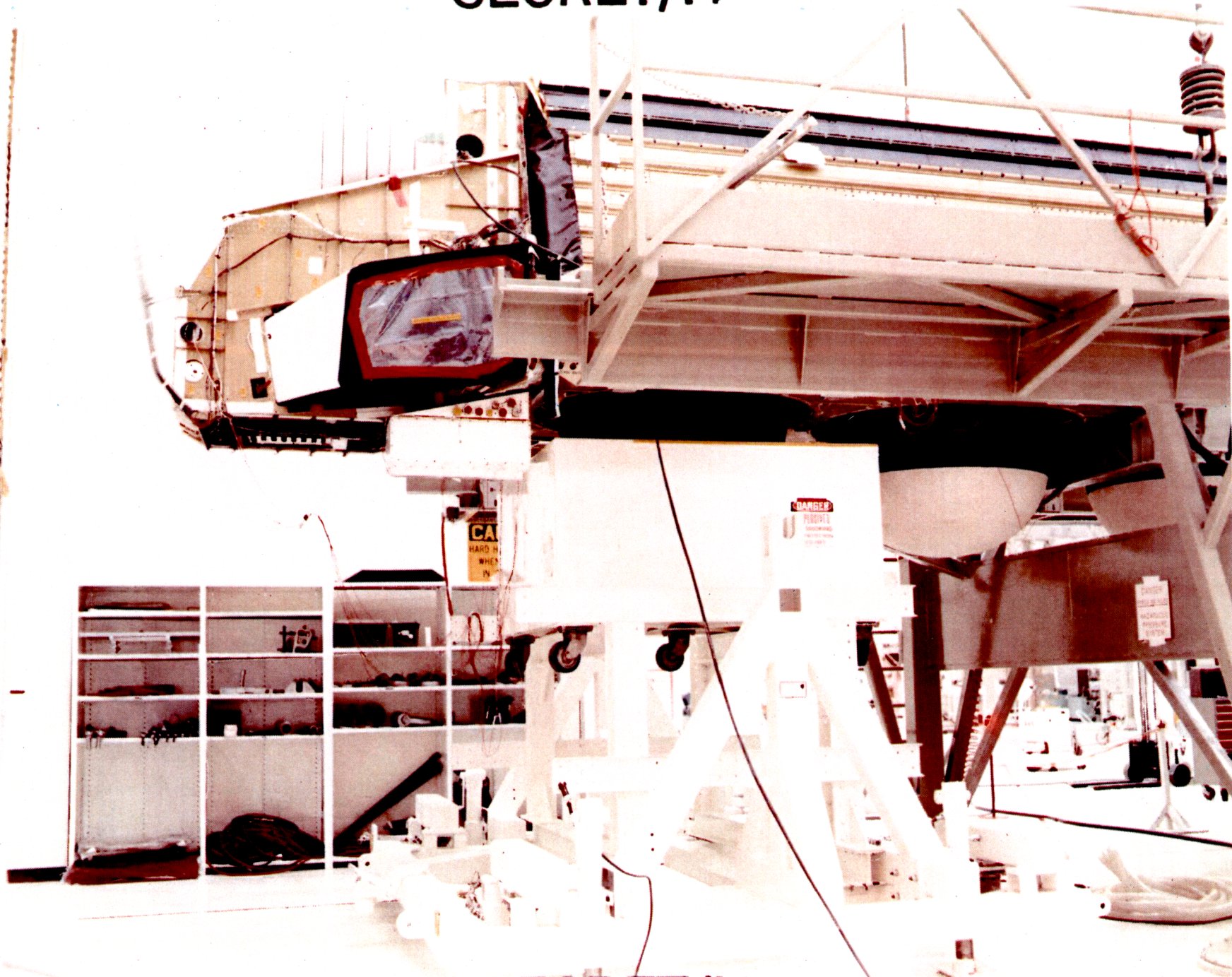
SV-5 Forward section with mapping camera module
